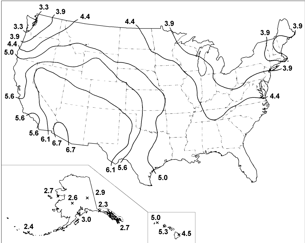
Figure 4. Average daily sunlight in kWh/m 2 [4, p. 187].
