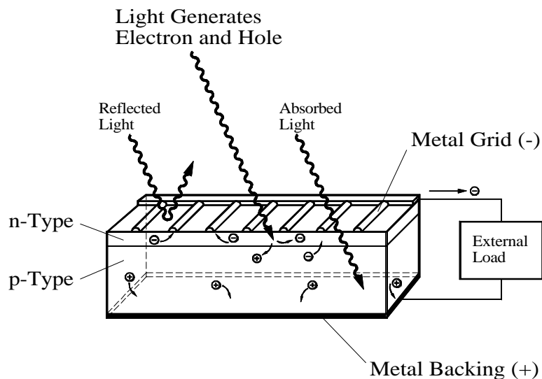
Figure 1. How solar cells work [4, p. 22].
