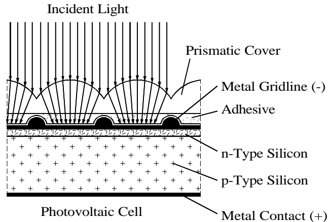
Figure 3. Prism cover for high-current solar cell [12].
