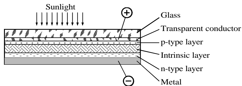
Figure 2. Typical thin-film amorphous silicon construction.
