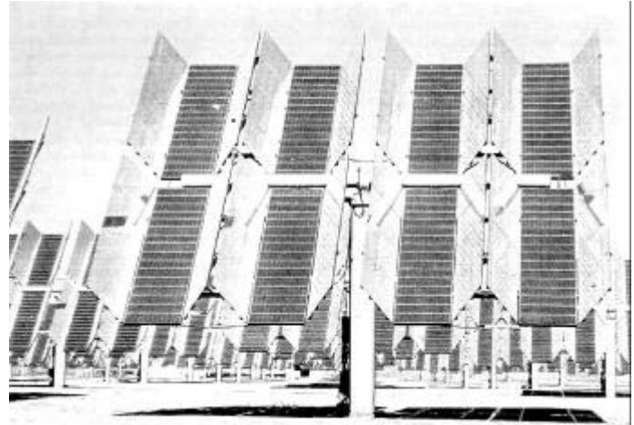
Figure 5. 6.5 MWp facility at Carissa Plains, California [26].
